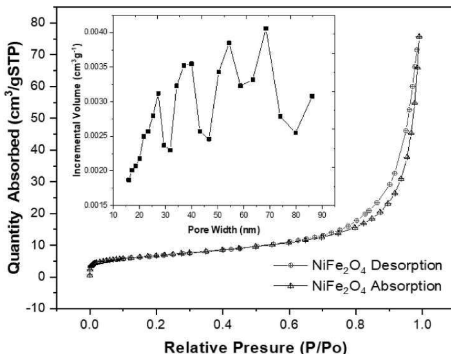
Fig. 2. BET analysis of \text{NiFe}_2\text{O}_4 catalyst.
