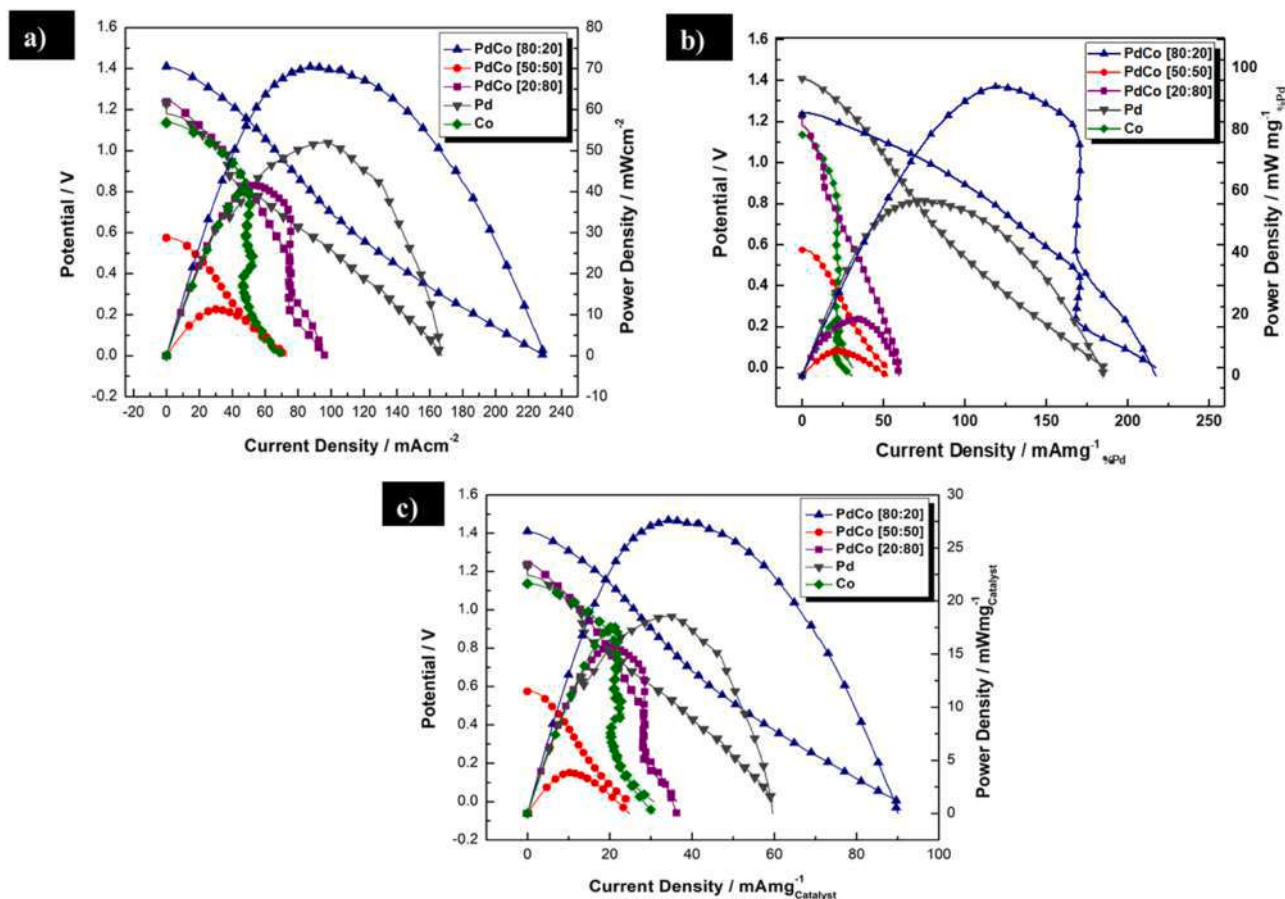
Fig. 8. MFC performance for PdCo, PdCo, PdCo, Pd, and Co aerogels in 0.5 M C_2H_6O and 0.5 M KOH at 10 \text{ mV s}^{-1} . Normalized by a) area, b) Pd mass according to XPS results and c) by mass of catalyst loaded.
