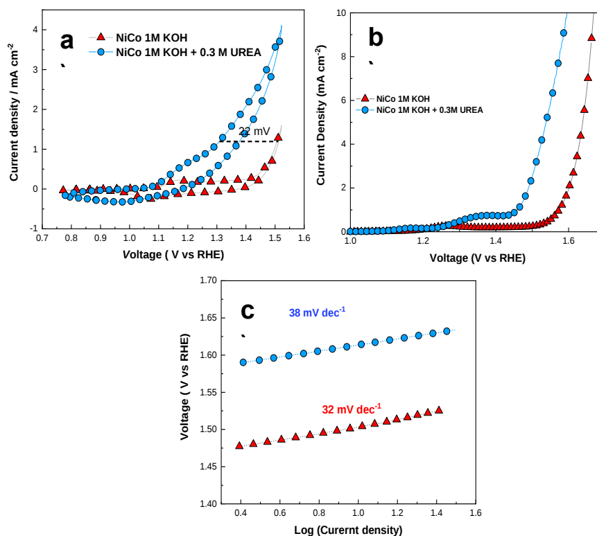
Figure 5. Electrochemical performance of the urea oxidation reaction (UOR).
