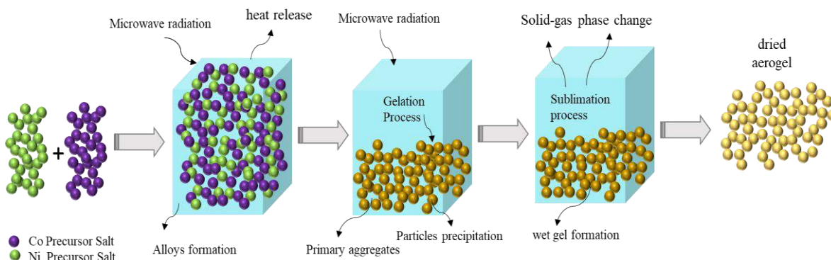
Figure 1. Synthesis process of NiCo aerogels.
