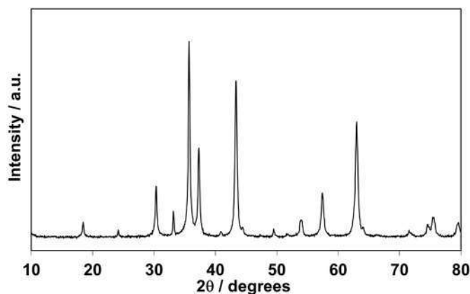
Fig. 1. XRD pattern of \text{NiFe}_2\text{O}_4 catalyst.
