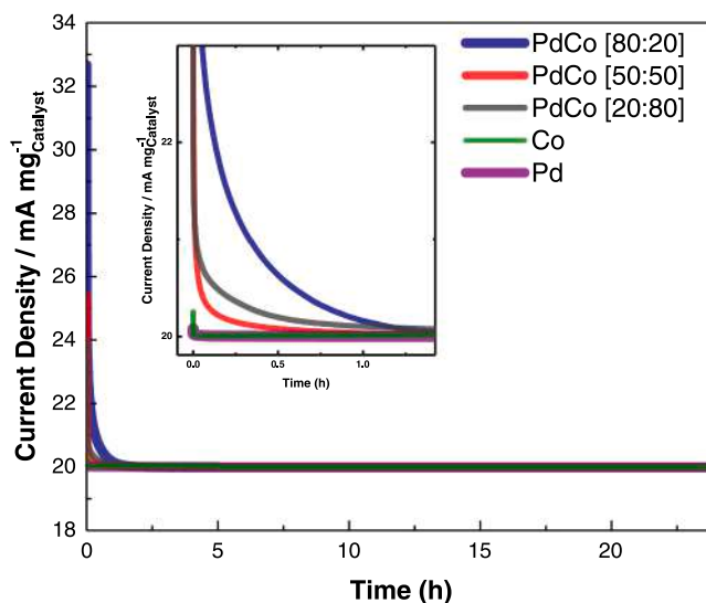
Fig. 7. Stability behavior for PdCo, Pd, and Co aerogels measured at 0.8 V vs. RHE in 0.5 M C 2 H 6 O and 0.5 M KOH.
