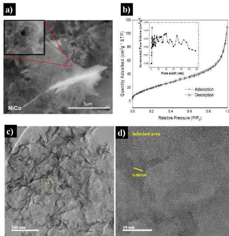
Figure 3. a) SEM images of NiCo aerogel; b) BET Analysis: isotherms and porosity of NiCo aerogel; c) and d) HR-TEM images of NiCo aerogel.
