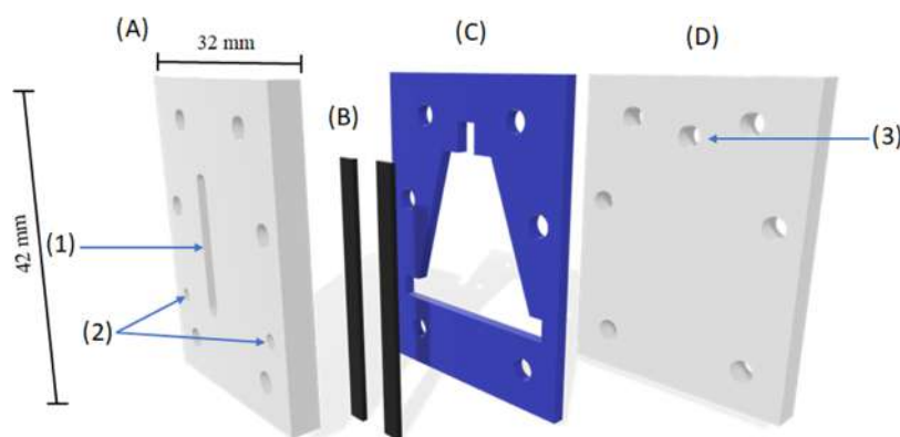
Figure 1. Microfluidic fuel cell (MFC)-type "Y" configuration. (A) Top cover, (B) carbon paper electrodes, (C) silastic gaskets, and (D) lower cover.
