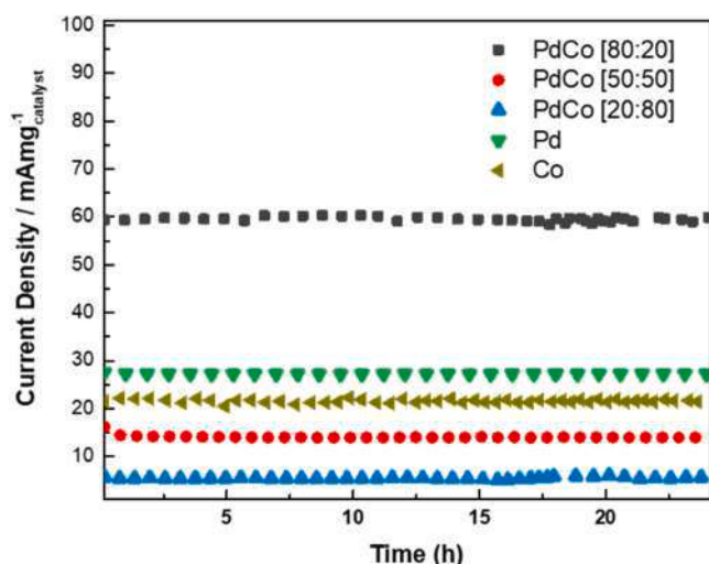
Fig. 9. MFC stability tests for aerogels measured at 0.8 V in 0.5 M ethanol + 0.5 M KOH.
