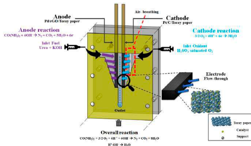
Scheme 1. Schematic illustration of the DUµFC configuration. The operation in flow-through electrolytes with independent inlets and the coupling of the catalysts.
