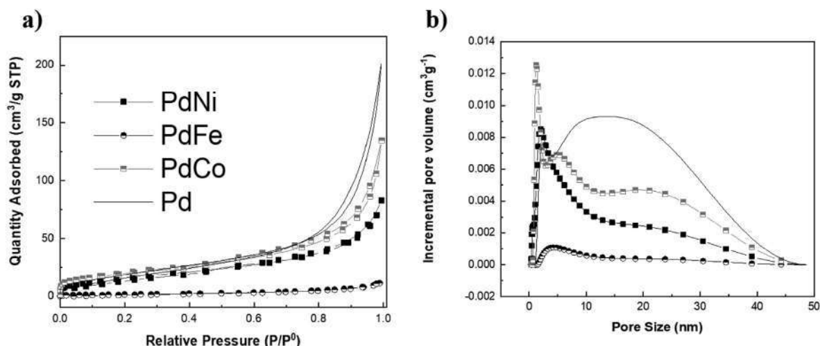
Fig. 3. a) N 2 adsorption-desorption isotherms for the synthesized Pd-TM aerogel samples b) Pore size distribution in the samples studied according to 2D-NLDFT model.
