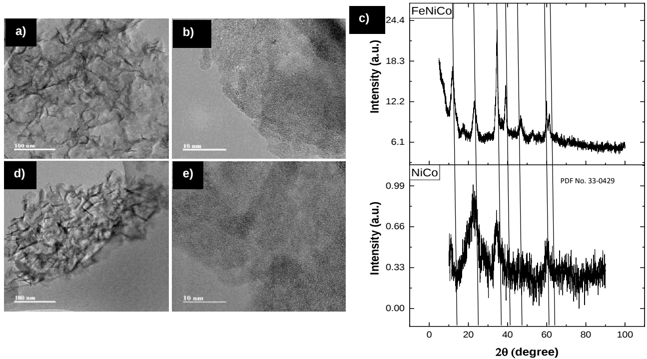
Fig. 2 Physico-chemical characterisations of aerogels: TEM images of (a-b) NiCo and (d-e) FeNiCo. XRD patterns of NiCo and FeNiCo.
