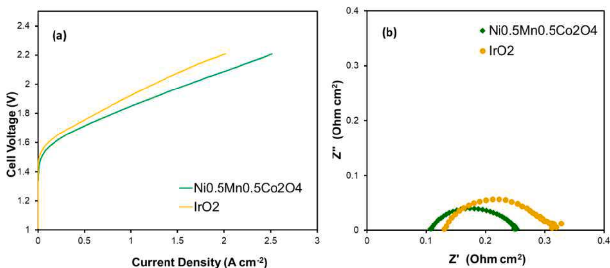
Fig. 7. (a) Performance and (b) EIS (at 1.8 V) data comparison at 60 °C for the cells equipped with Ni_{0.5}Mn_{0.5}Co_2O_4 and commercial IrO_2 at the anode, in 1 M KOH as supporting electrolyte.
