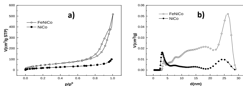
Fig. 1 N 2 isotherms using the BET technique: a) N 2 adsorption-desorption, b) Porosity analysis.
