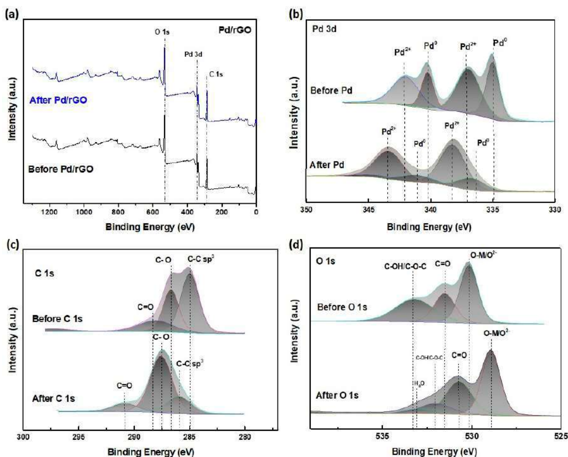
Figure 2. Comparison of high-resolution XPS of Pd/rGO before and after evaluation of DUμFC performance. (a) General spectra of Pd/rGO; (b) spectra in the Pd 3d; (c) spectra in the C 1s region; and (d) spectra in the O 1s region.
