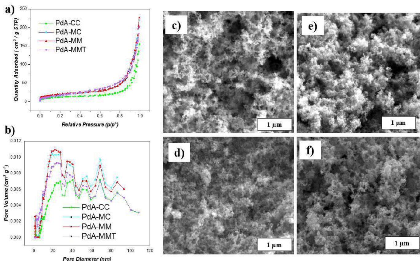
Figure 5. Physicochemical analysis. BET analysis of Pd aerogels: (a) \text{N}_2 adsorption isotherms; and (b) pore size distribution. SEM of Pd aerogels: (c) PdA-CC; (d) PdA-MC; (e) PdA-MM; and (f) PdA-MMT.
