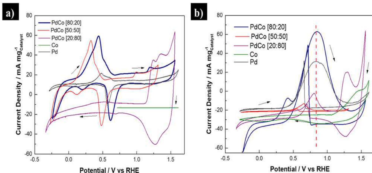
Fig. 6. a) CVs for PdCo, Pd and Co aerogels at 50 mV s -1 in 0.5 M KOH. b) EOR activity for PdCo, Pd and Co aerogels at 50 mV s -1 in 0.5 M C 2 H 6 O and 0.5 M KOH.
