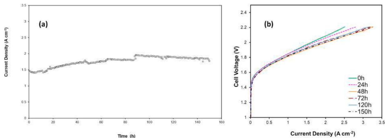
Fig. 8. (a) Chronoamperometric test for the cell equipped with \text{Ni}_{0.5}\text{Mn}_{0.5}\text{Co}_2\text{O}_4 at 60 °C and 2 V; (b) J-V curves at 60 °C during the time-stability test, feeding 1 M KOH solution as supporting electrolyte.
