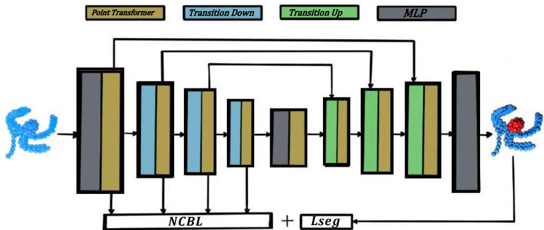
Figura 6.3. Nested Contrastive Boundary Learning Point Transformer (NCBL-PT). Imagen propia.
